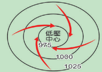
南半球氣旋
